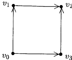
Figure 1: An orientation of a 4-cycle
