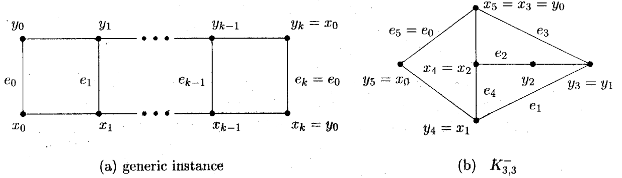
Figure 2: Möbius sequences
